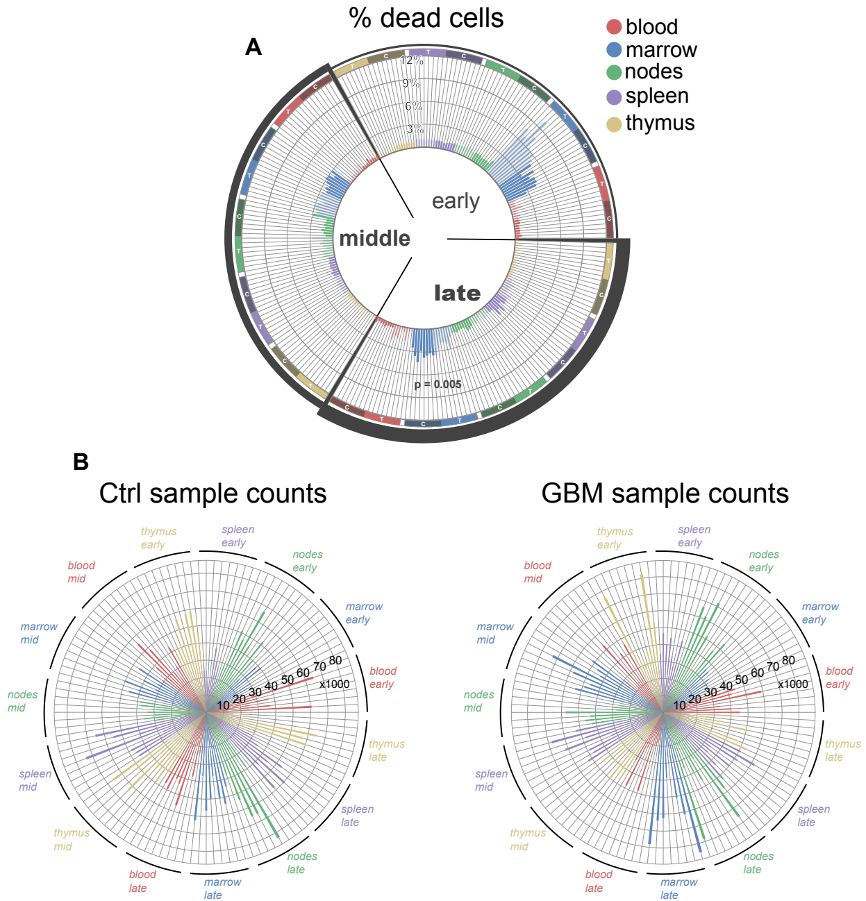
Fig. S3. Cell Viability and Sample Counts for the 240 Lymphoid Tissues Analyzed in this Study, Related to Fig. 1. (A) Radial bar chart showing the percentage of dead cells among the dataset's 240 tissue samples. C = control samples, T = GBM samples. Viability only differed between the two groups in the bone marrow at the t = 30-day time point ( p = 0.005 , two-tailed independent Student's t test, n = 8 mice/group). (B) Radial bar charts showing the number of cells in control (left) and GBM (right) mouse tissue samples after weighted random sampling by tissue to balance the number of cells per sample.
